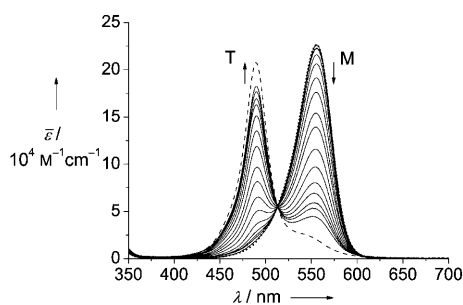
Figure 2. Concentration-dependent UV/Vis spectra of 2 ( c = 3 \times 10^{-4} to 1 \times 10^{-6} M) in \text{CHCl}_3 at 298 K. The arrows indicate the decrease in the intensity of the monomer band (M; ..... ) and the appearance of the trimeric aggregate band (T; ----) with increasing concentration. The spectra of pure monomeric dyes and the pure trimer aggregates were derived from the data at two different concentrations and the aggregation constants.
